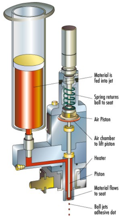
Jet Applicator Cutaway View
