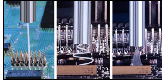
Bead, Monofilament, Spray Patterns
