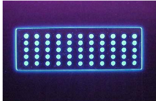
2.5mm Acrylic Dots Jetted on Glass Slide
