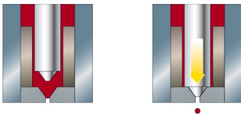
Needle Impacting Seat Ejects Droplet
