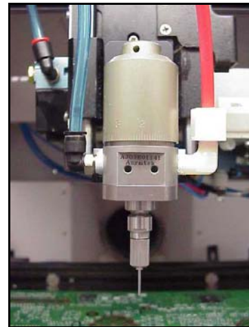
Hybrid Needle-Jet Applicator
