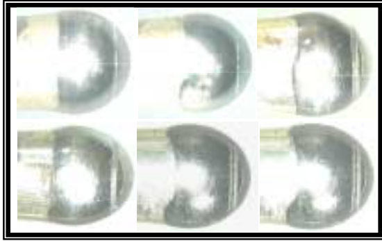
Figure 11. Needle head wearout from jetting abrasive underfill material.
