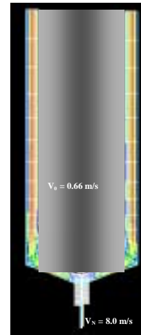
Figure 3. Resultant velocities from numerical calculations.
