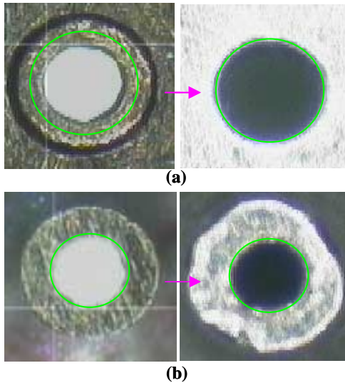
Figure 13. Nozzle wearout progress resulted from jetting abrasive materials: (a) Interior end of nozzle diameter. (b) Nozzle outside orifice.
