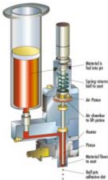
other parameter that affected fluid properties was the nozzle heater temperature setting. Figure 1. Diagram of the cross section of Asymtek DJ-2111 Jet
