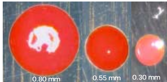
among different SMA dot sizes jetted onto a metal plate. Figure 7. Different SMA dot sizes jetted onto a metal finishing plate
