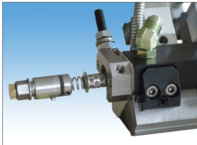
Replaceable quick-change filter cartridge helps deliver precise, clean applications.
