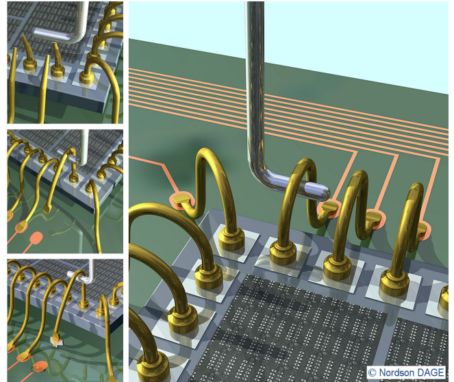
Wire pull bond test
