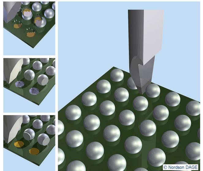
Ball shear test
